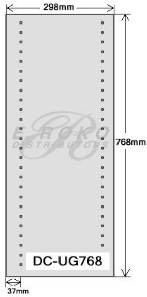
30" UPPER GABLE
