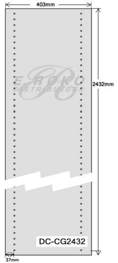
96" CLOSET GABLE
