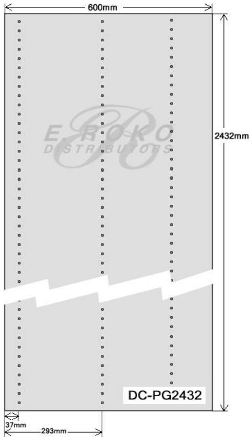
96" PANTRY GABLE
